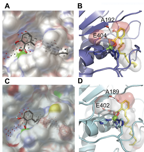
Fig. 5. Predicted binding mode of anacardic acid to gelatinase. A, surface diagram of the docked structure of anacardic acid into the MMP-2 active site, with the AutoLigand fill points on a 1-Å grid spacing. The gray points represent optimal locations for carbon atoms, and the red points represent optimal locations for hydrogen bond acceptor atoms. B, ribbon structure of MMP-2 with the docked structure of anacardic acid shown in sticks. The large green sphere is the coordinated zinc atom and the transparent surface surrounding anacardic acid represents the AutoLigand optimized binding pocket. Hydrogen bonding is depicted as black dashed lines. C, surface diagram of docked structure of anacardic acid into the MMP-9 active site. D, ribbon structure of MMP-9 with docked structure of anacardic acid shown in sticks. Surface diagram figures were generated using PMV ( http://mglttools.scripps.edu ); ribbon diagrams were generated by PyMOL ( http://www.pymol.org ).
