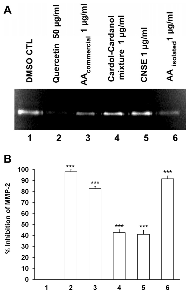
Fig. 2. Regulation of MMP-2 activity by components of CNSE. A, zymogram showing MMP-2 activity of conditioned media from 3T3-L1 fibroblast cells treated with 0.5% DMSO (lane 1), quercetin at 50 \mu\text{g/ml} (lane 2), commercial anacardic acid (AA) (Calbiochem) (lane 3), the cardol-cardanol mixture (lane 4), CNSE (lane 5), and anacardic acid isolated from CNSE (lane 6), each at 1 \mu\text{g/ml} . B, a representative plot of percentage inhibition observed in the zymogram. Each bar represents the mean \pm S.E. of triplicate determinations from three independent experiments. ***, P < 0.001 (one-way analysis of variance with Dunnett's multiple-comparison post-test). CTL, control.
