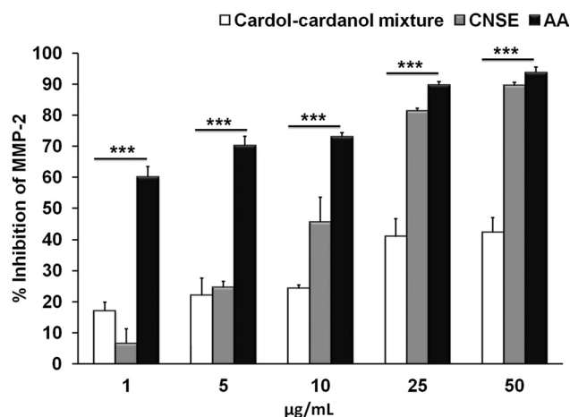
Fig. 4. Fluorescence-based studies on MMP-2 inhibition by CNSE components. Plot shows percentage inhibition of the MMP-2 catalytic core domain in the presence of different concentrations of CNSE, the cardol-cardanol mixture, and anacardic acid isolated from CNSE (at a concentration range of 1 to 50 µg/ml). *** P < 0.001 (one-way analysis of variance).
